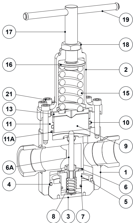
1 1/2" and 2" – DN 40 and DN 50
